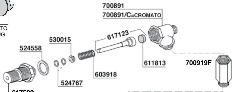
617523 617523/C=CROMATO FILETTO PASSO 2 mm PITCH THREAD 2 mm
