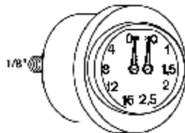
620406 150 Lt/h 620406/X 150 Lt/h INOX-STAINLESS STEEL 620406/2 200 Lt/h 620406/1 100 Lt/h
