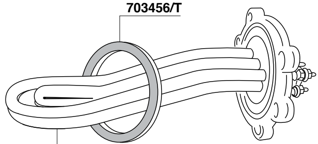
703457/22 =GR1 230V 1800W 150mm 703457/11 =GR1 115V 1500W 155mm 703467 =GR2 230/400V 2700W 230/400V 175mm 703458 =GR2 230/400V 3000W 340mm 703478 =GR2 230/400V 4500W 340mm 703459 =GR3/4 230/400V 5000W 570mm
