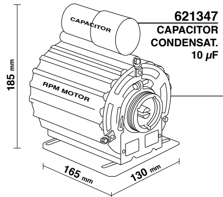
700084/22 V220/50/60 W165 HP0,2 WITH CABLE
