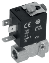
Ø 1,6 1/8F-1/8F 616602/11 V120-110/50-60 616602/22 V230/50 616602/24 V230/50
