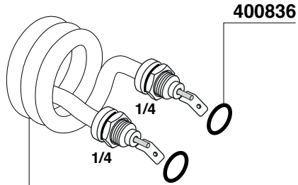
400625 1200W 220V Ø55 mm.68 400626 1200W 110V Ø55 mm.68
