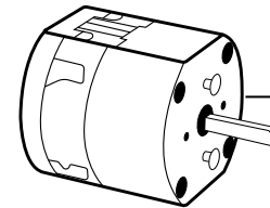
700154/22=V220/50 W165 HP0,2 170x165x185 mm
